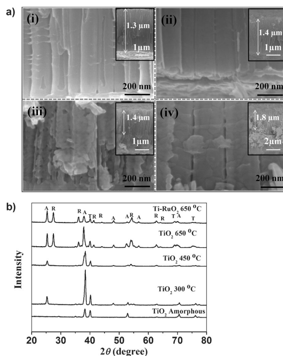
Figure 2. a) SEM images of self-organized \text{TiO}_2 nanotubes and ruthenium-doped \text{TiO}_2 nanotubes formed by electrochemical anodization and annealed for 1 h at i) 300 °C, ii) 450 °C, iii) 650 °C, and iv) Ru- \text{TiO}_2 at 650 °C. b) X-ray diffraction patterns for \text{TiO}_2 nanotubes and Ru-doped \text{TiO}_2 nanotubes of (a) after some annealing treatments. T = Ti substrate, A = anatase, R = rutile.
