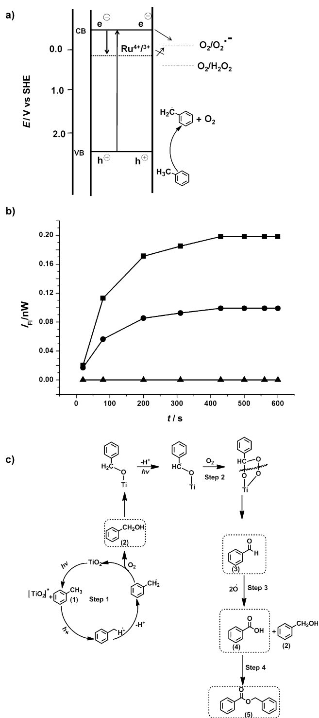
Figure 3. a) Illustration of the band position during toluene oxidation on TiO_2 (anatase and rutile) and ruthenium-doped TiO_2 nanotubes under UV irradiation. CB = conduction band, VB = valence band. b) Fluorescence intensity as a function of time at different samples. ■ anatase TiO_2 , ● rutile TiO_2 , ▲ Ru-rutile TiO_2 . c) The proposed reaction pathways during photocatalytic toluene oxidation.
